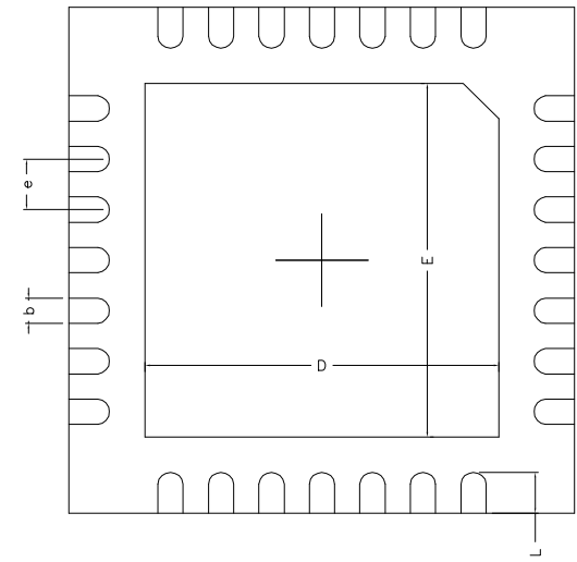
BOTTEM VIEW
