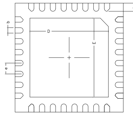
BOTTEM VIEW
