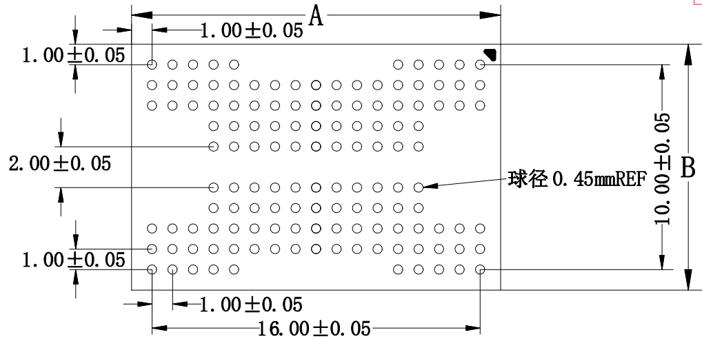
BOTTOM VIEW
